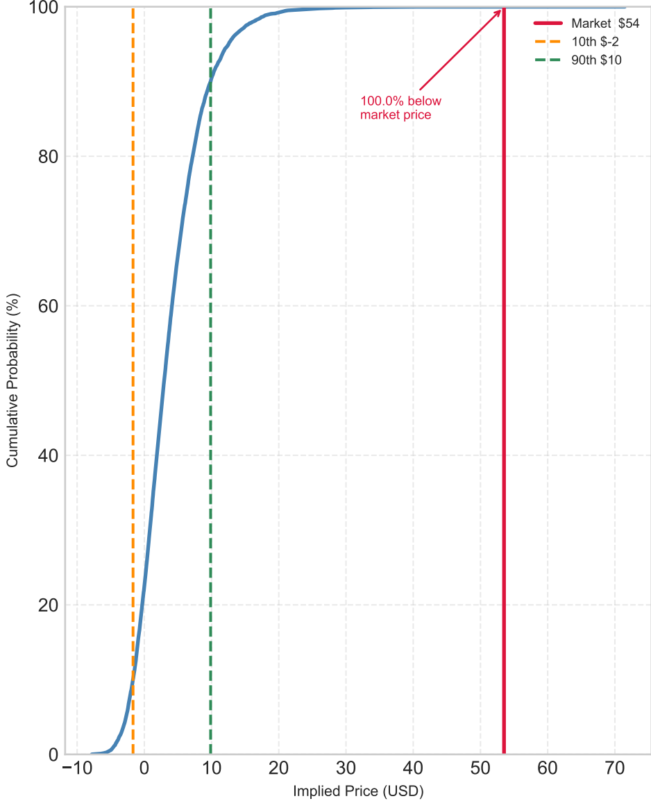
Cumulative Distribution
