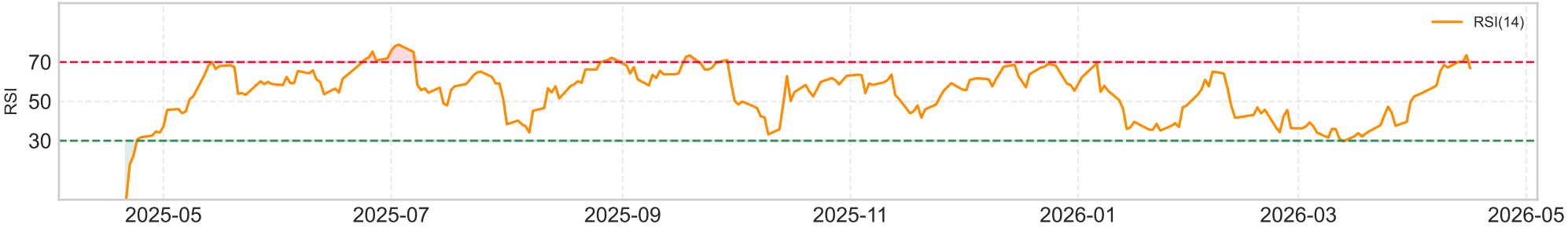
RSI (14-day Wilder) — Current: 66.8 [NEUTRAL]
