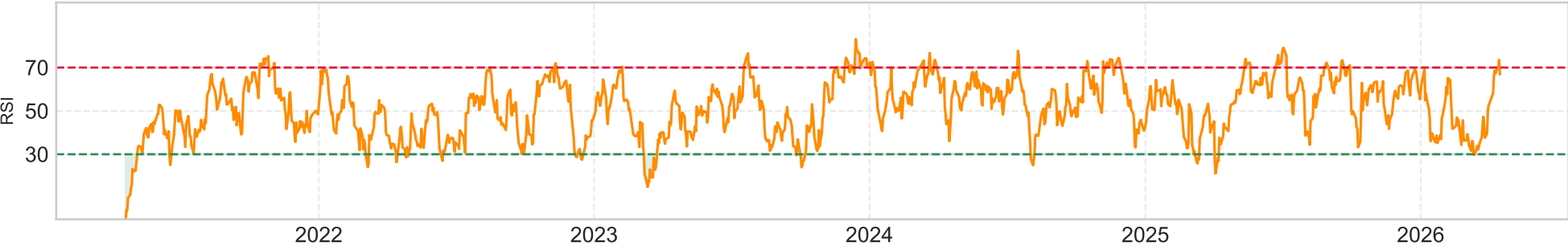
RSI (14-day) — Current: 66.8
